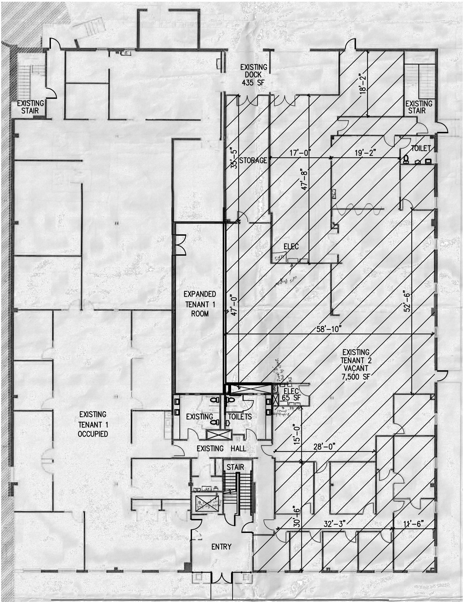
EXISTING FIRST FLOOR VACANT 2 PLAN SCALE: 1/16"=1'-0"
